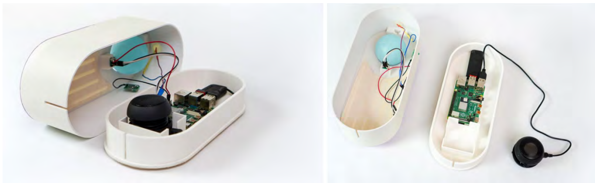
Figure 4: Broadcast is comprised of a Raspberry Pi microcontroller, a small speaker, and a 20-pin rotary encoder attached to the blue resin sphere.
